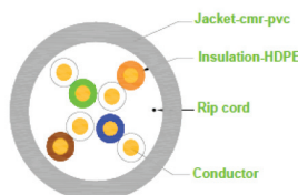
Part No. T5eUTP-CMR-GY-CF
